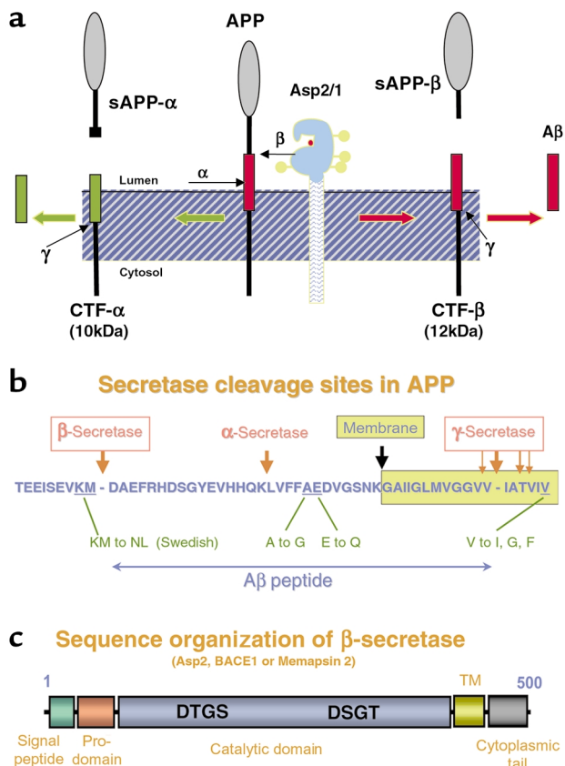
Figure 1 APP processing pathway and domain organization of \beta -secretase. (a) A schematic representation of the sequential cleavages of APP at the \beta - and \gamma - sites to generate \beta -amyloid. APP and \beta -secretase are both integral membrane proteins with type 1 orientation, \gamma -secretase is probably PS 1, a protein with eight TM domains (not shown). Recent data indicates that these three proteins assemble in conjunction with Nicastrin, a protein which interacts with PS1, in cholesterol rich microdomains in cellular membranes. (b) The amyloid domain of APP showing the mutations which are associated with early onset familial forms of AD, highlighting those which occur at the secretase cleavage sites. The beginning of the TM domain is shown. (c) Domain organization of \beta -secretase. The protein has a cleaved signal peptide, a prodomain and a catalytic domain in which the catalytic aspartic residues are located. The catalytic domain shows the 3 di-sulfide bridges characteristic of the pepsin family of aspartic proteinases and is glycosylated at 4 sites. The cytoplasmic tail contains a di-leucine endosomal retrieval signal, cysteine residues which are palmitoylated and phosphorylation sites. The homolog, Asp1 (DRAP, BACE2) shows the same overall structural organization.
